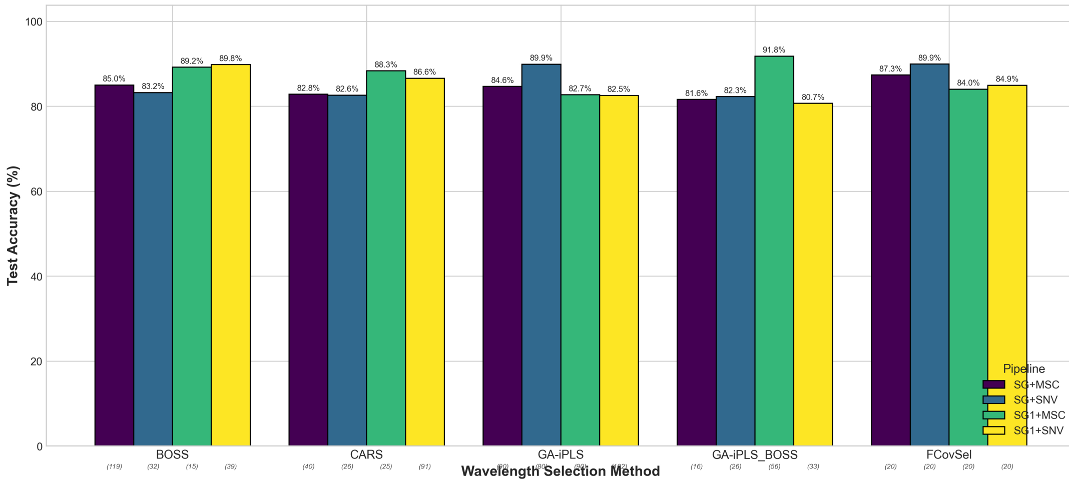
3D-CNN Test Accuracy by Wavelength Selection Method & Preprocessing (Salinas) (Number of selected bands shown in parentheses)
